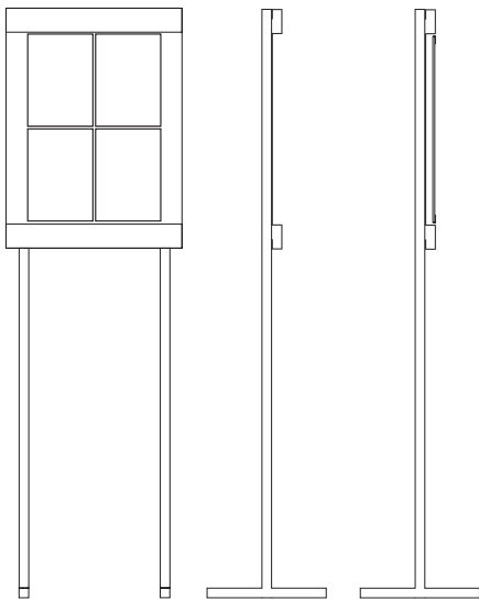
delhi 400 [4 x A4] w 550 x h 1800 x d 500mm w 21,65 x h 70,87 x d 19,69"
