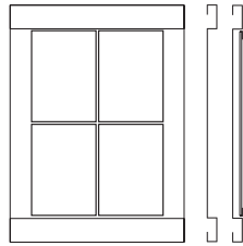
delhi 400 [4 x A4] w 550 x h 750 x d 30mm w 21,65 x h 29,53 x d 1,18"
