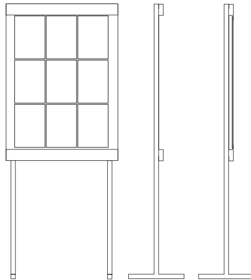
delhi 900 [9 x A4] w 750 x h 1800 x d 500mm w 29,53 x h 70,87 x d 19,69"
